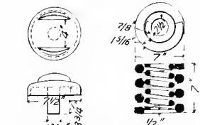
Figs. 4764-4765. Spring-caps (4).
